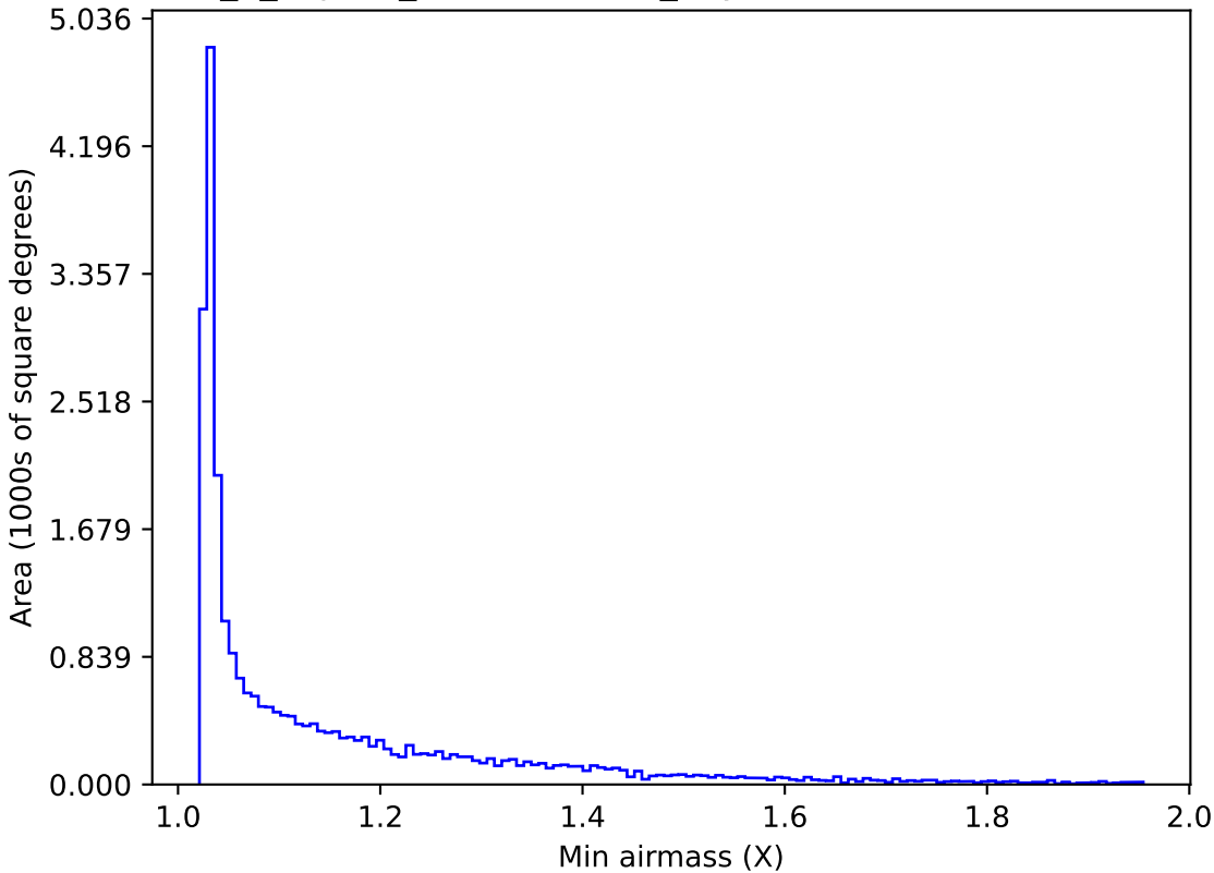
internal_u_expt60_nscale1.1v3.4_10yrs Yr 1 all bands: Min airmass
