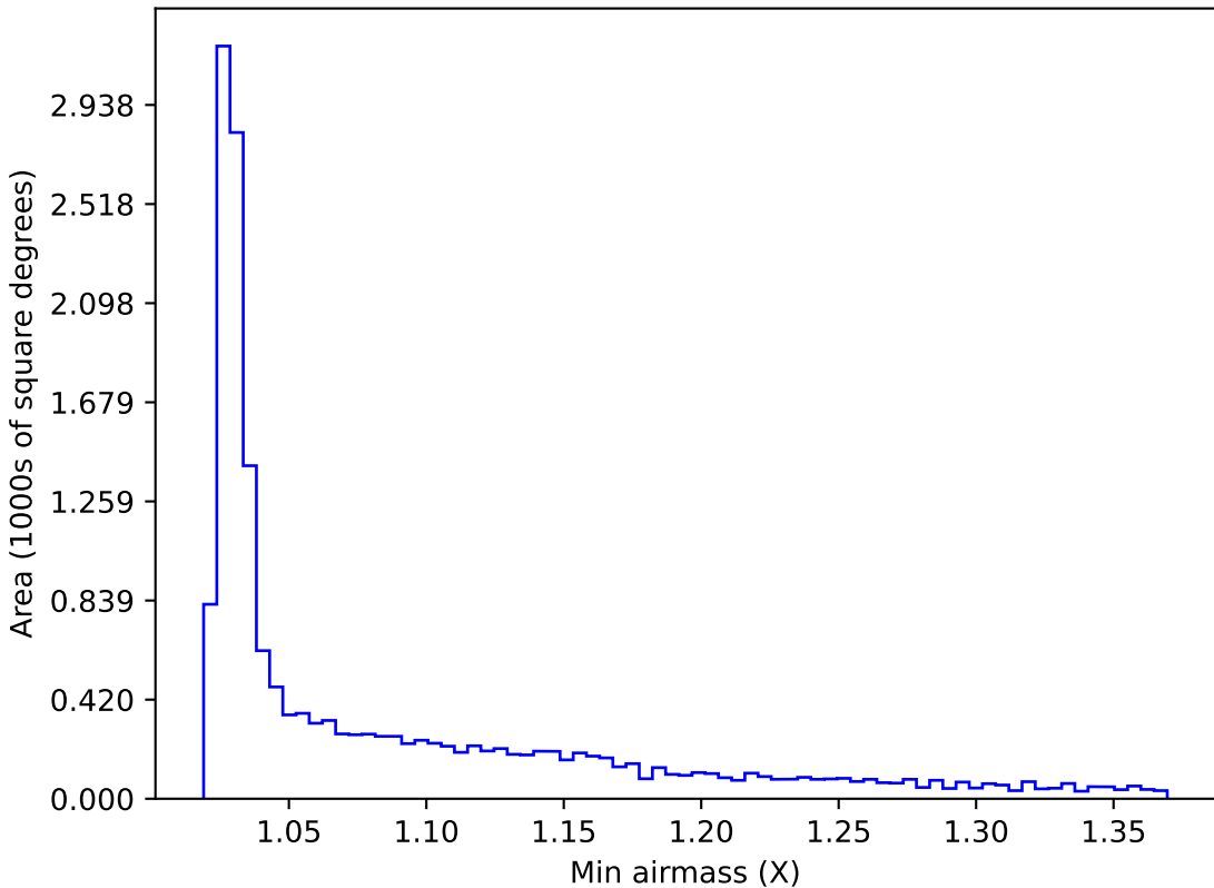
internal_u_expt60_nscale1.1v3.4_10yrs WFD z band: Min airmass
