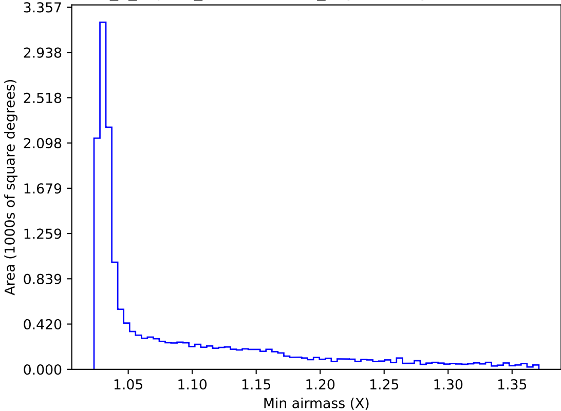
internal_u_expt60_nscale1.1v3.4_10yrs WFD y band: Min airmass
