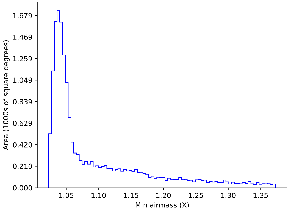
internal_u_expt60_nscale1.1v3.4_10yrs WFD u band: Min airmass
