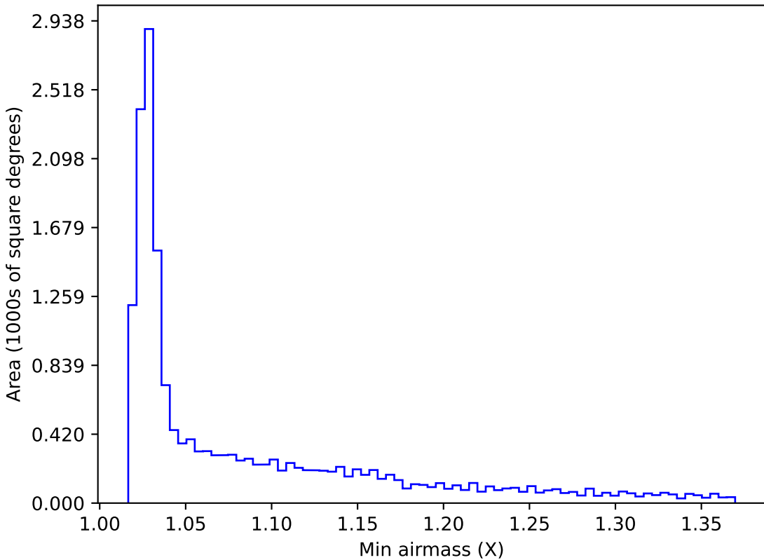
internal_u_expt60_nscale1.1v3.4_10yrs WFD r band: Min airmass
