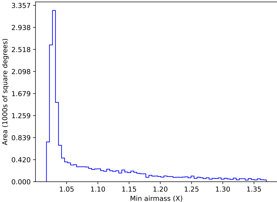
internal_u_expt60_nscale1.1v3.4_10yrs WFD i band: Min airmass
