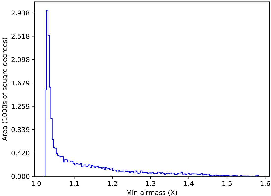
internal_u_expt60_nscale1.1v3.4_10yrs All sky y band: Min airmass
