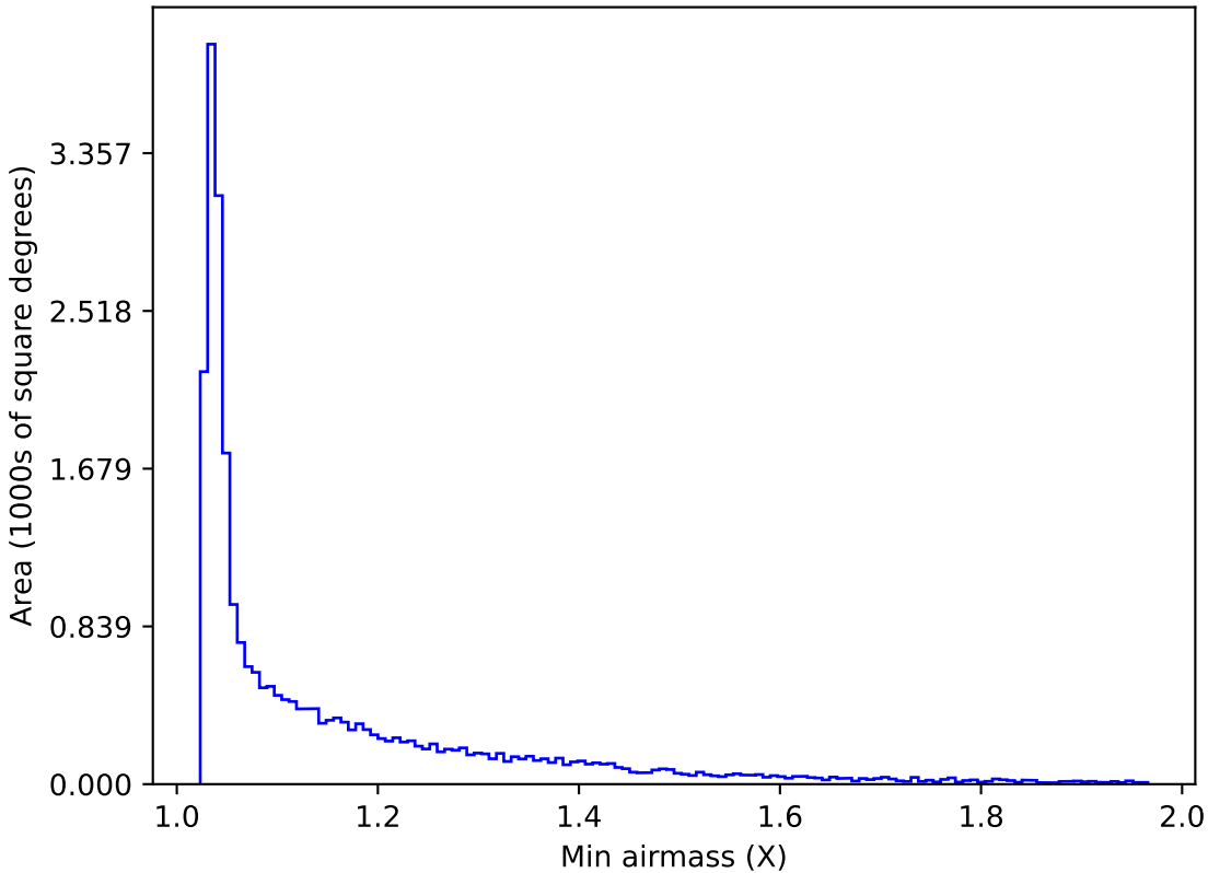
internal_u_expt60_nscale1.1v3.4_10yrs All sky g band: Min airmass
