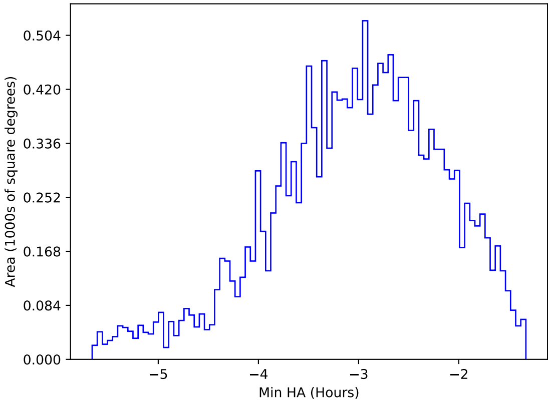
internal_u_expt60_nscale1.1v3.4_10yrs WFD u band: Min HA
