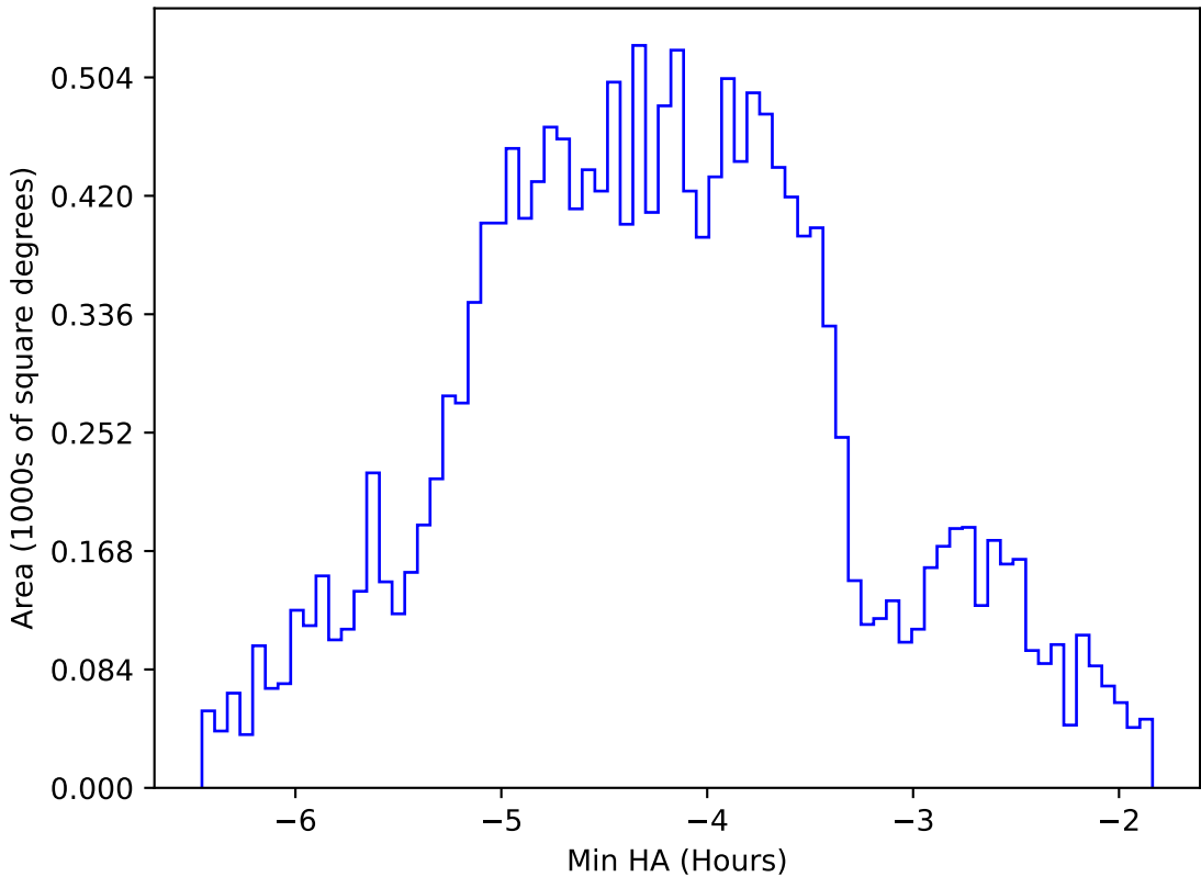
internal_u_expt60_nscale1.1v3.4_10yrs WFD g band: Min HA
