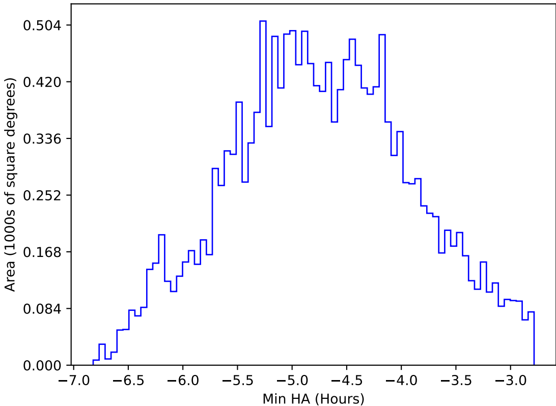
internal_u_expt60_nscale1.1v3.4_10yrs WFD all bands: Min HA
