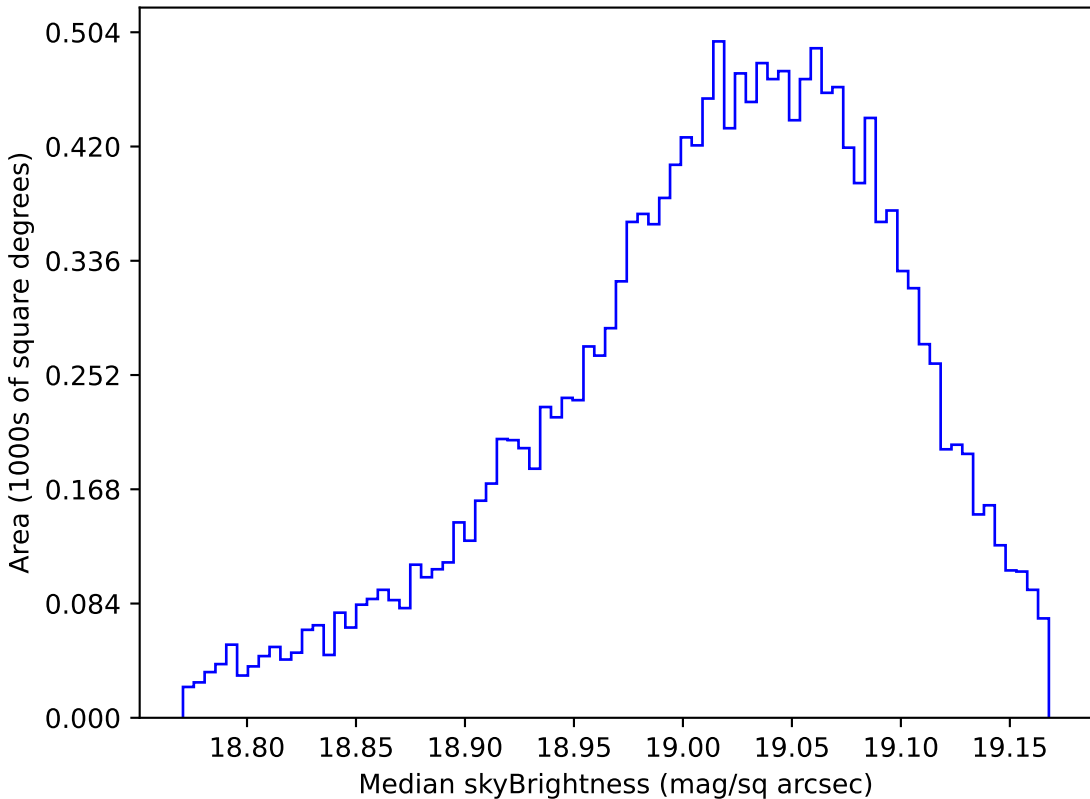
internal_u_expt60_nscale1.1v3.4_10yrs WFD z band: Median skyBrightness
