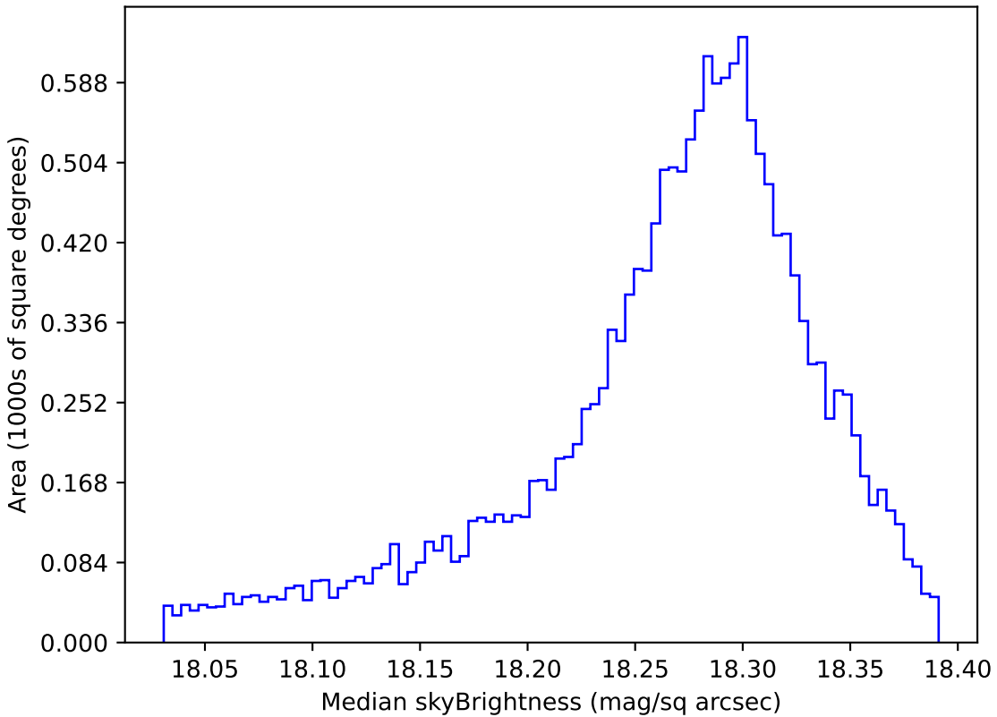
internal_u_expt60_nscale1.1v3.4_10yrs WFD y band: Median skyBrightness
