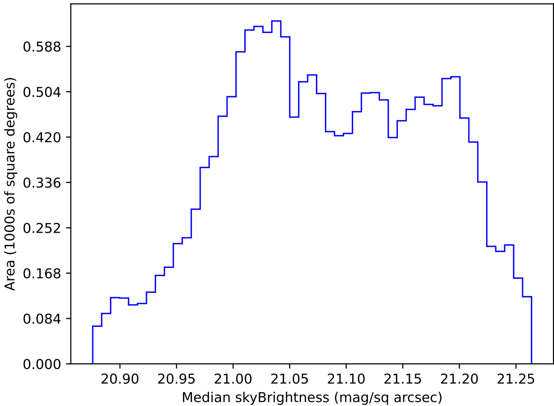
internal_u_expt60_nscale1.1v3.4_10yrs WFD r band: Median skyBrightness
