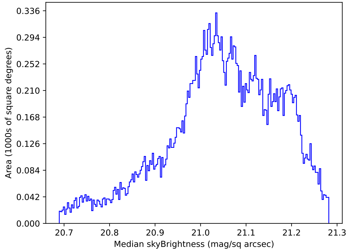
internal_u_expt60_nscale1.1v3.4_10yrs All sky r band: Median skyBrightness
