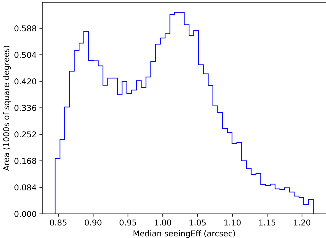
internal_u_expt60_nscale1.1v3.4_10yrs WFD i band: Median seeingEff
