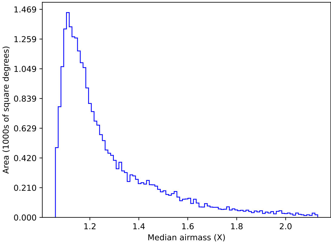
internal_u_expt60_nscale1.1v3.4_10yrs Yr 1 g band: Median airmass
