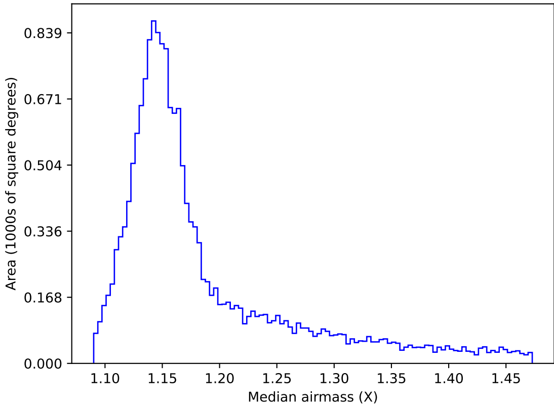
internal_u_expt60_nscale1.1v3.4_10yrs WFD y band: Median airmass
