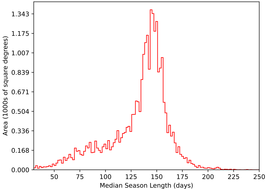
internal_u_expt60_nscale1.1v3.4_10yrs All sky i band: Median Season Length
