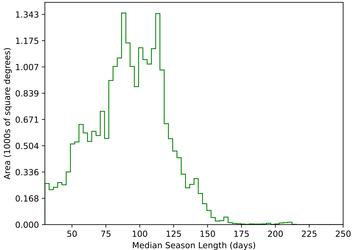
internal_u_expt60_nscale1.1v3.4_10yrs All sky g band: Median Season Length
