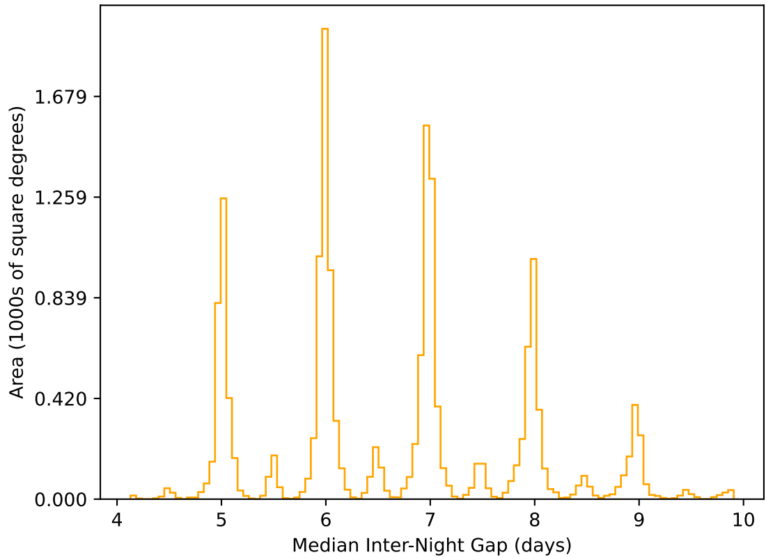
internal_u_expt60_nscale1.1v3.4_10yrs WFD r band: Median Inter-Night Gap
