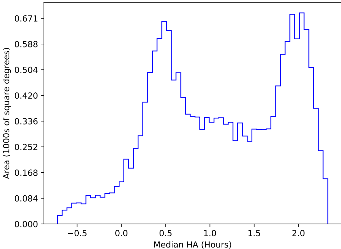
internal_u_expt60_nscale1.1v3.4_10yrs WFD z band: Median HA
