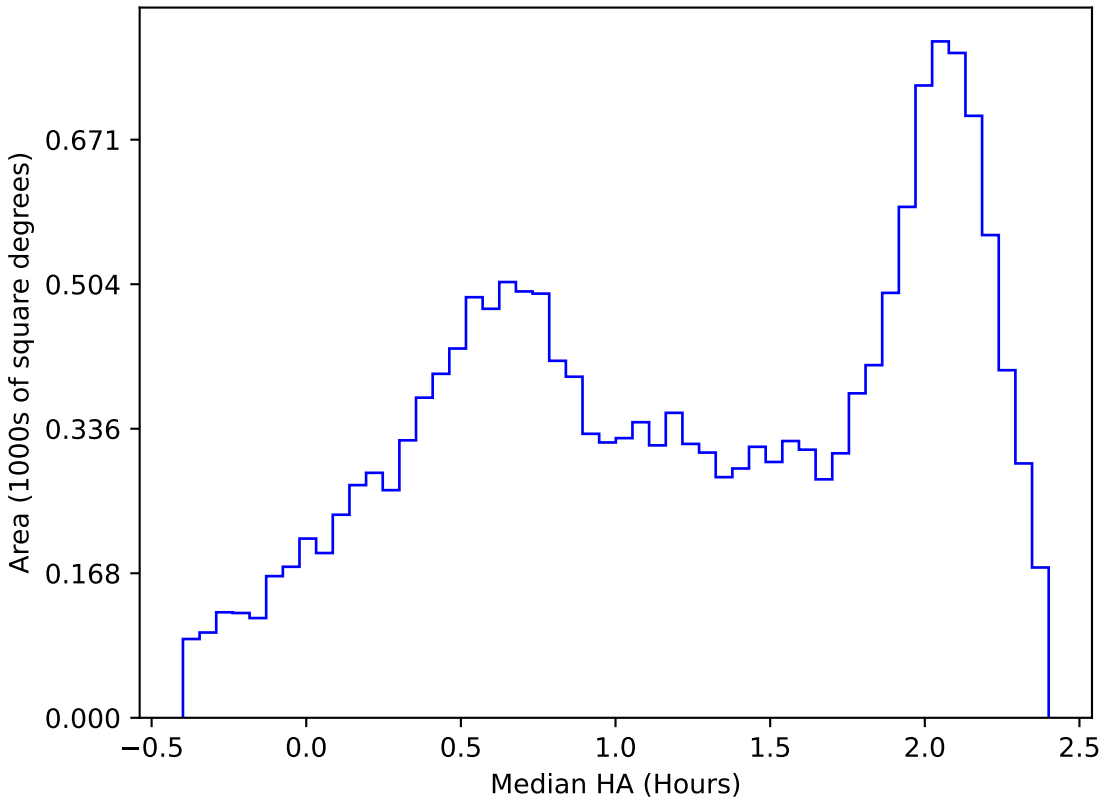
internal_u_expt60_nscale1.1v3.4_10yrs WFD y band: Median HA
