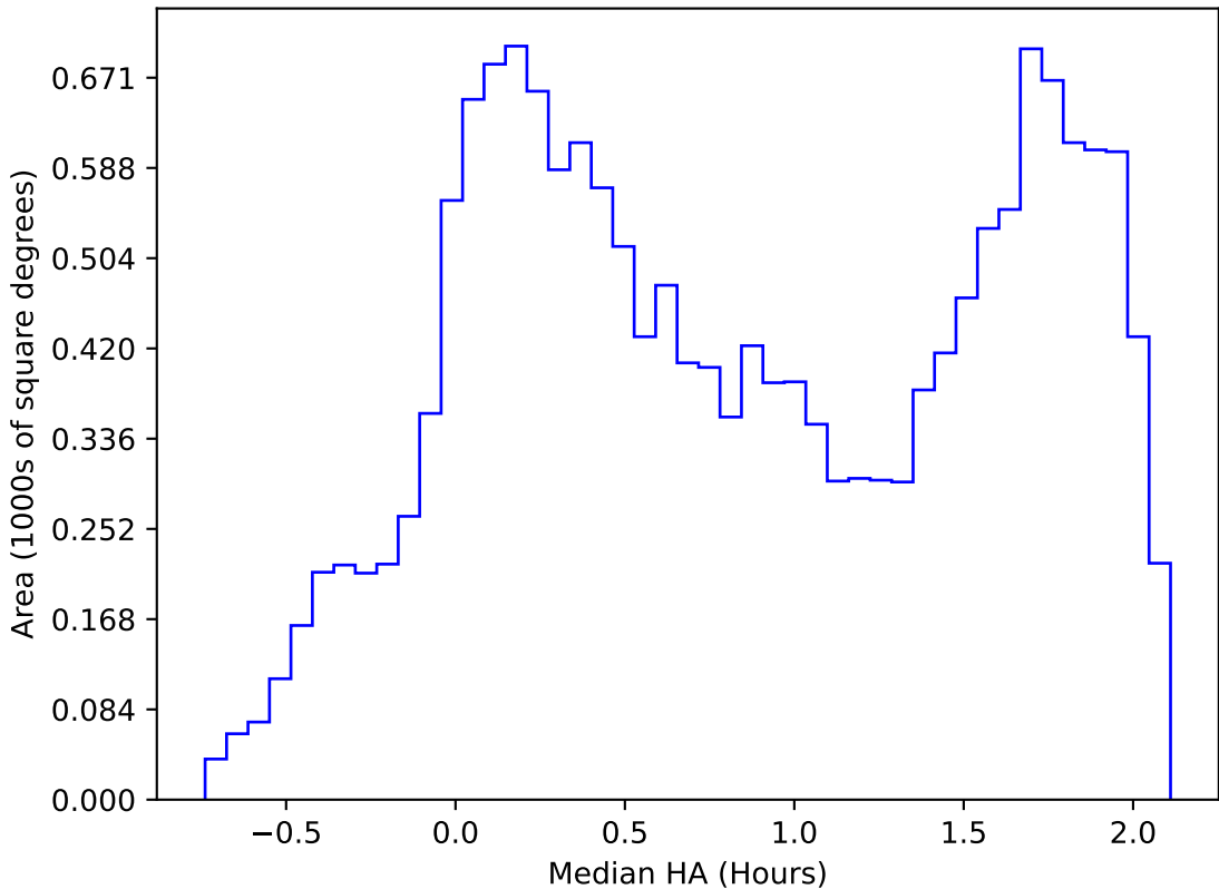
internal_u_expt60_nscale1.1v3.4_10yrs WFD r band: Median HA
