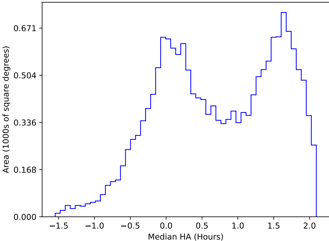
internal_u_expt60_nscale1.1v3.4_10yrs WFD g band: Median HA
