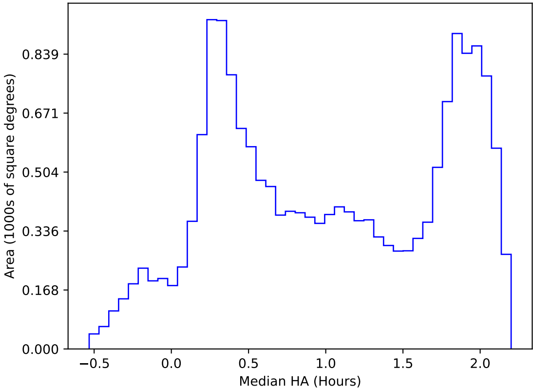
internal_u_expt60_nscale1.1v3.4_10yrs WFD all bands: Median HA
