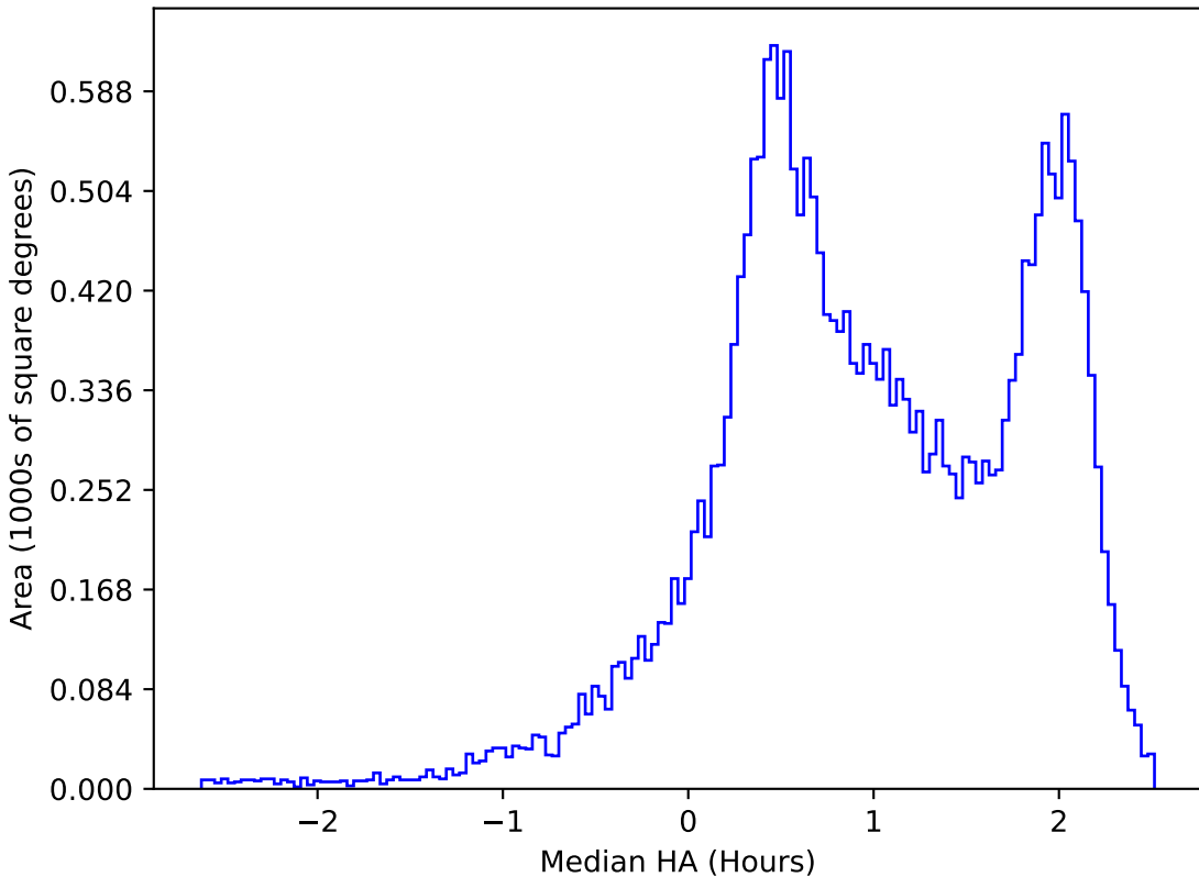
internal_u_expt60_nscale1.1v3.4_10yrs All sky z band: Median HA
