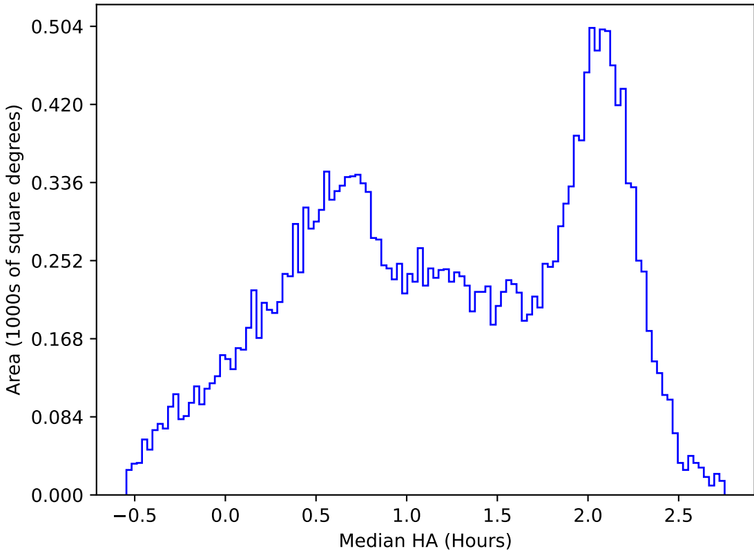
internal_u_expt60_nscale1.1v3.4_10yrs All sky y band: Median HA
