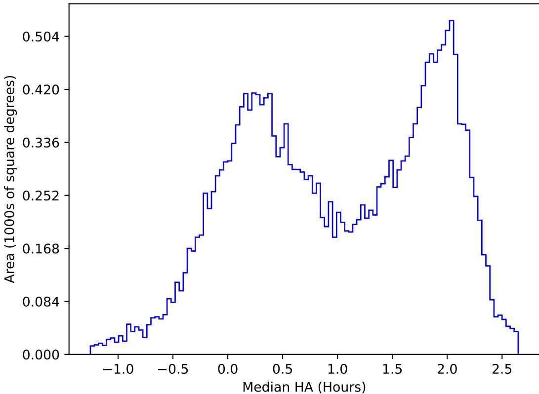
internal_u_expt60_nscale1.1v3.4_10yrs All sky u band: Median HA
