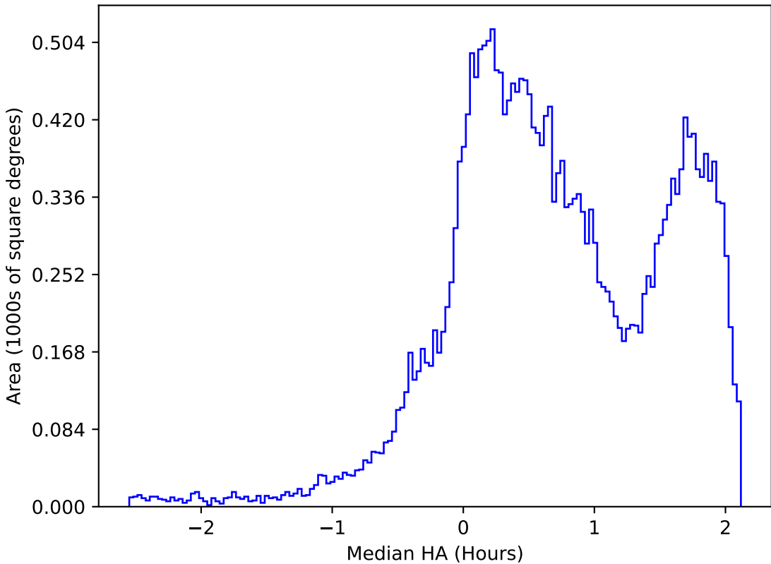
internal_u_expt60_nscale1.1v3.4_10yrs All sky r band: Median HA
