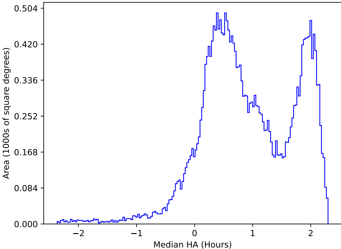
internal_u_expt60_nscale1.1v3.4_10yrs All sky i band: Median HA
