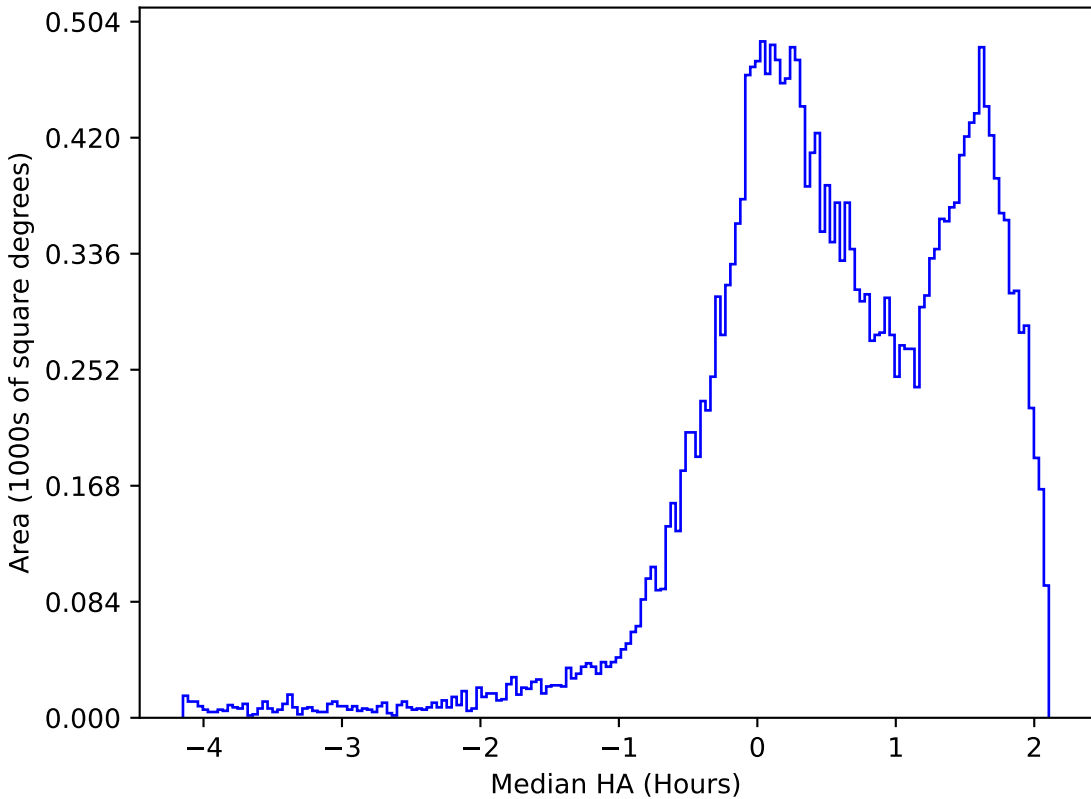
internal_u_expt60_nscale1.1v3.4_10yrs All sky g band: Median HA
