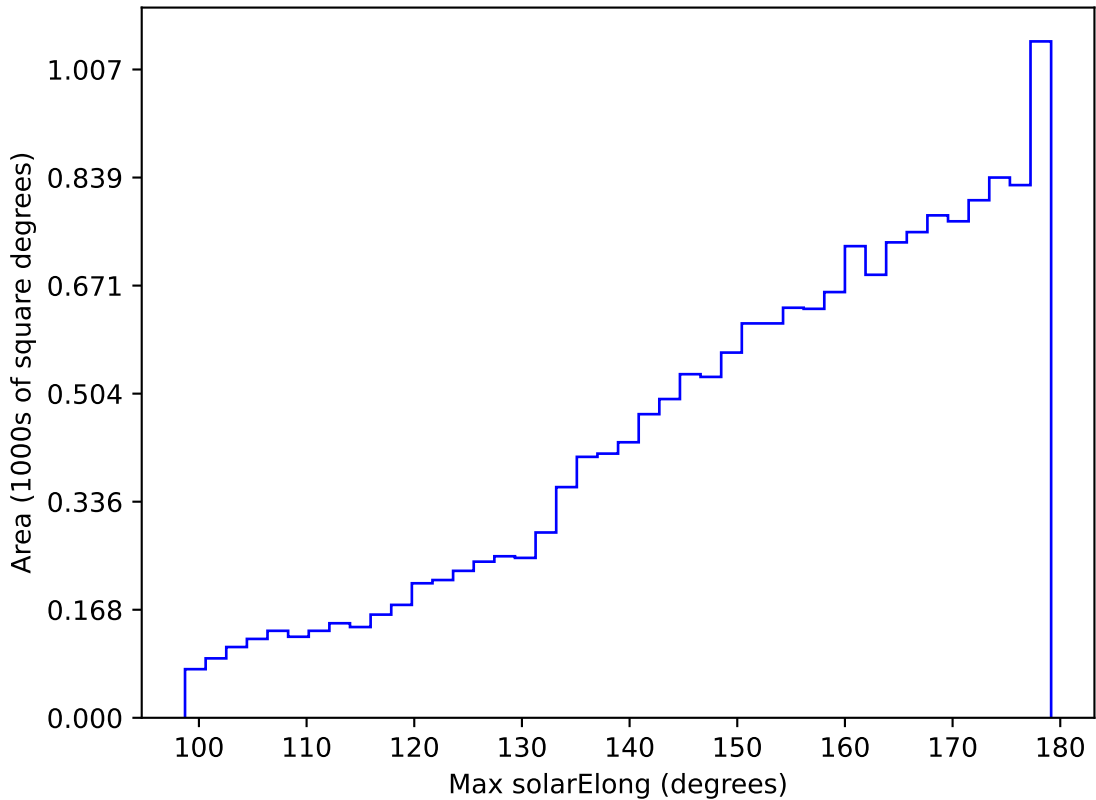
internal_u_expt60_nscale1.1v3.4_10yrs WFD y band: Max solarElong
