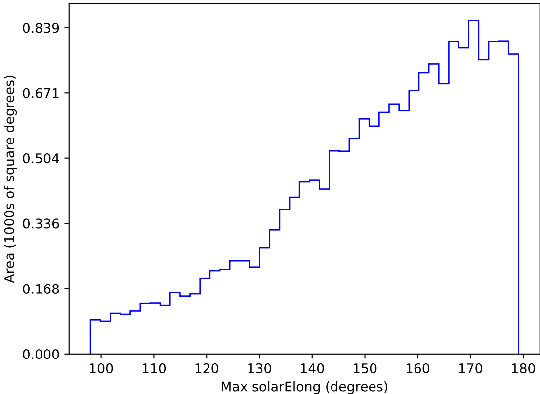
internal_u_expt60_nscale1.1v3.4_10yrs WFD u band: Max solarElong
