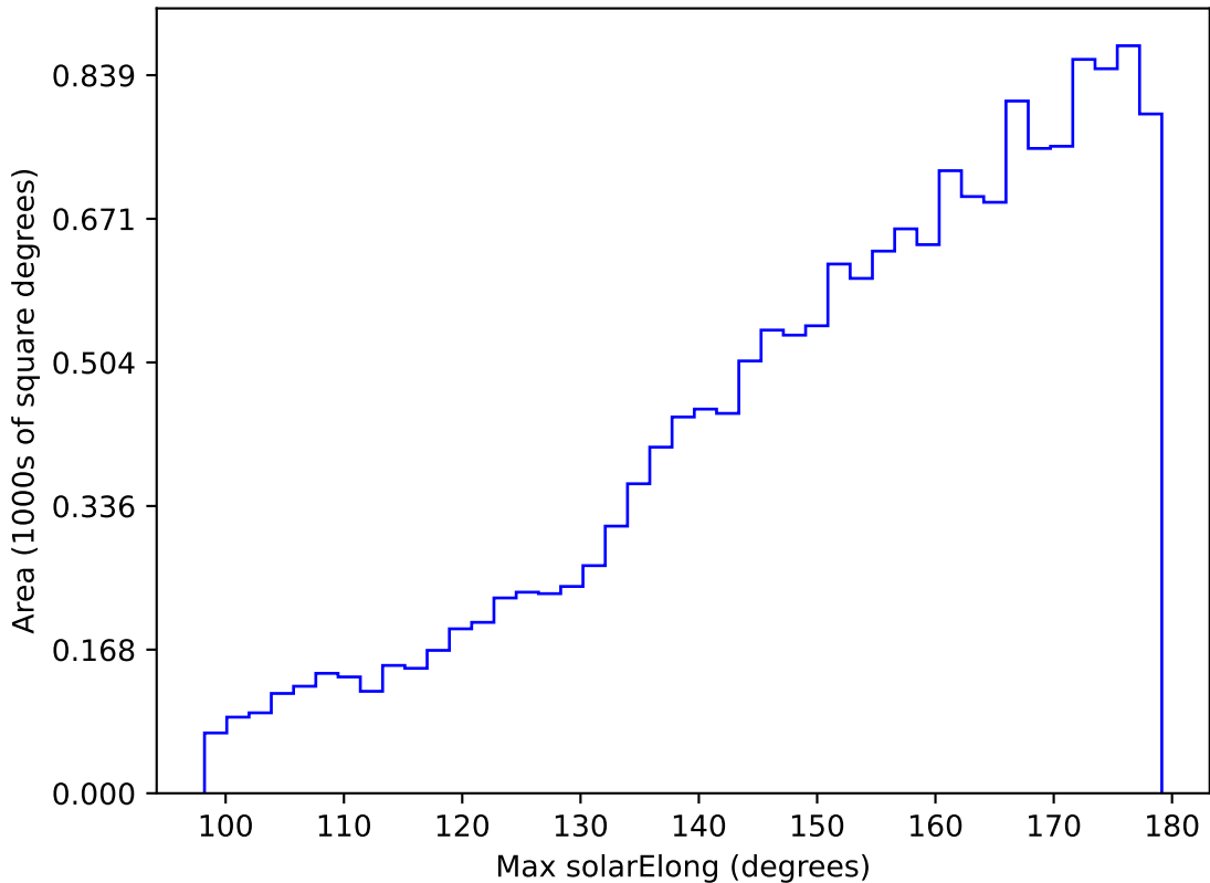
internal_u_expt60_nscale1.1v3.4_10yrs WFD g band: Max solarElong
