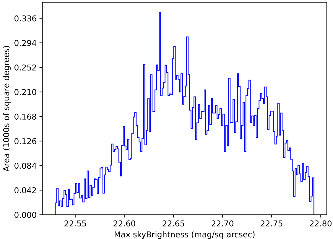
internal_u_expt60_nscale1.1v3.4_10yrs Yr 1 u band: Max skyBrightness
