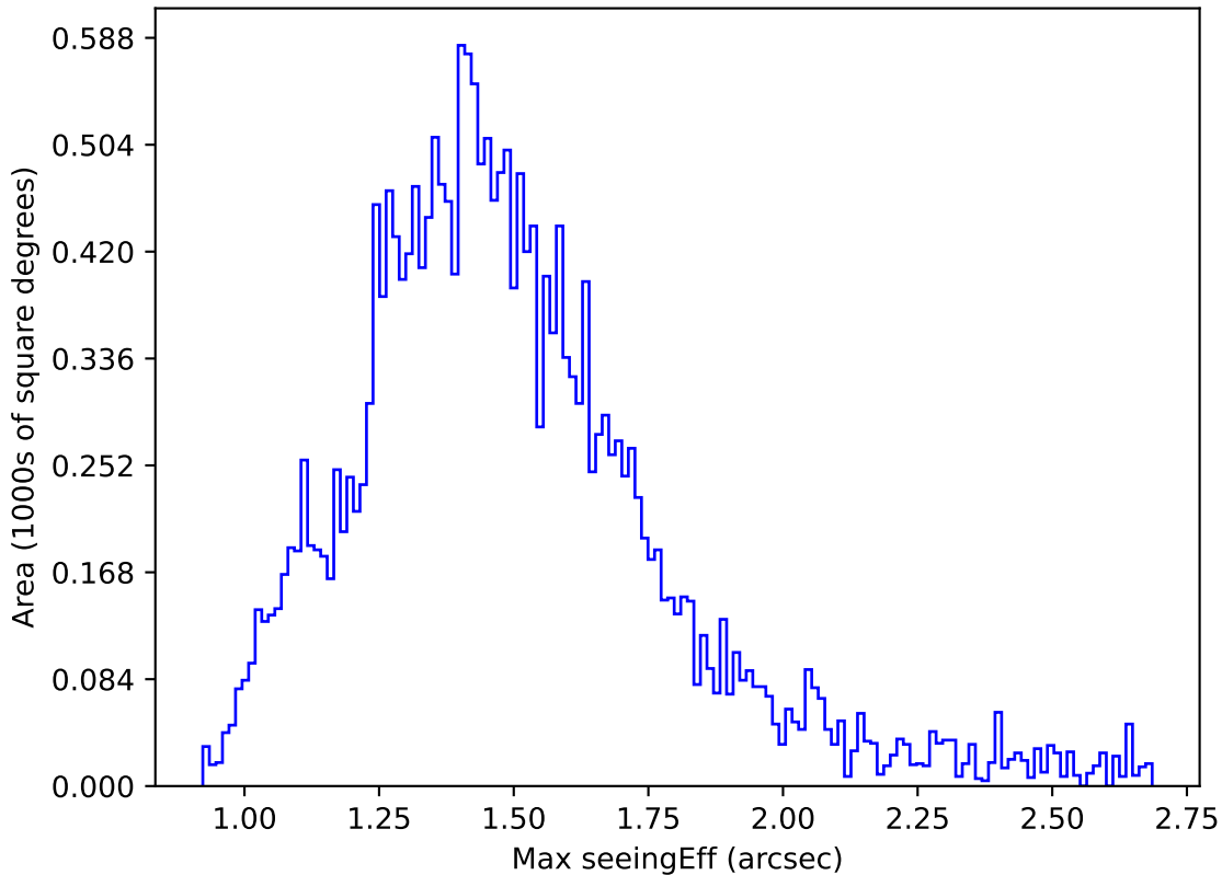
internal_u_expt60_nscale1.1v3.4_10yrs Yr 1 y band: Max seeingEff
