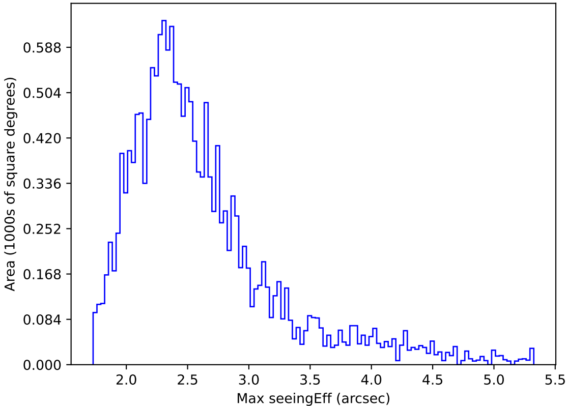
internal_u_expt60_nscale1.1v3.4_10yrs WFD z band: Max seeingEff
