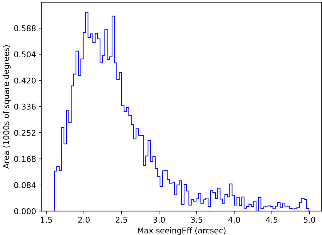
internal_u_expt60_nscale1.1v3.4_10yrs WFD y band: Max seeingEff
