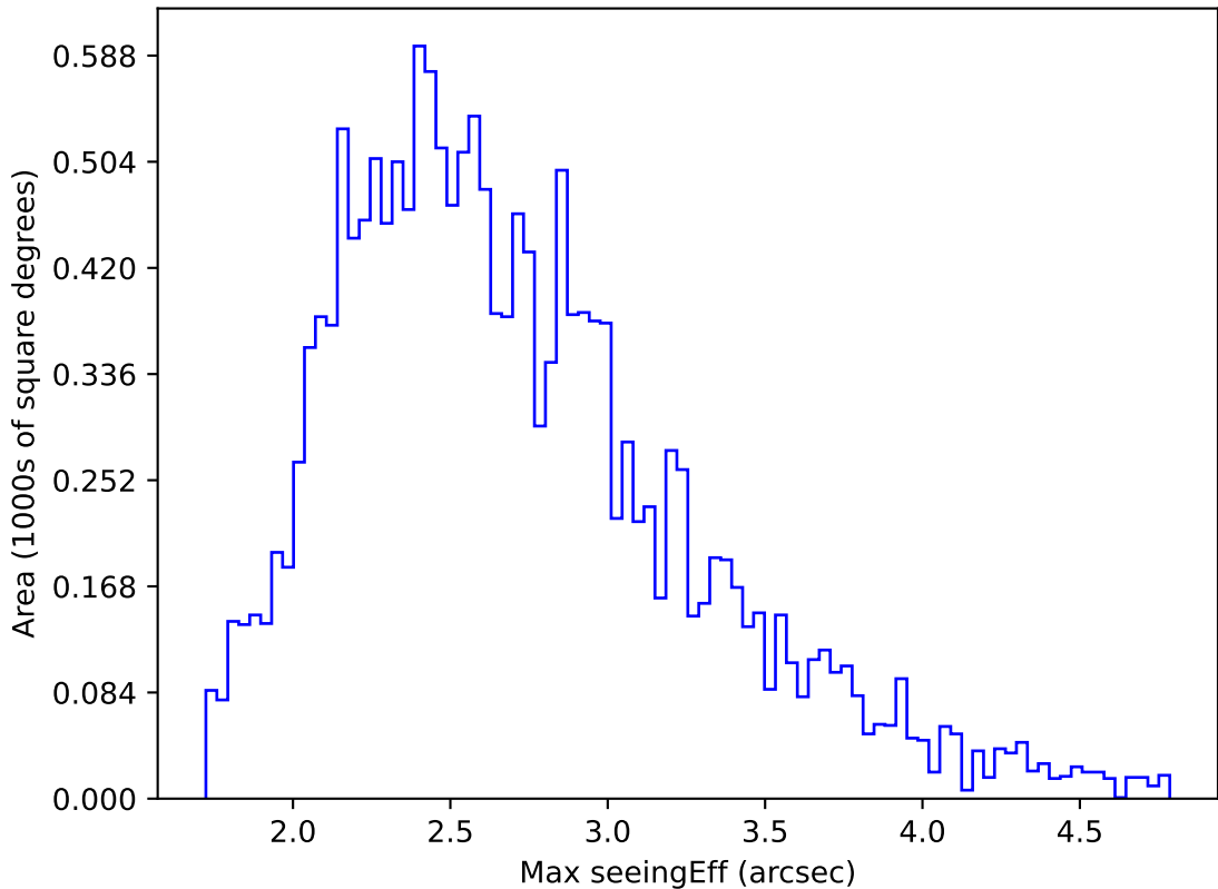
internal_u_expt60_nscale1.1v3.4_10yrs WFD i band: Max seeingEff
