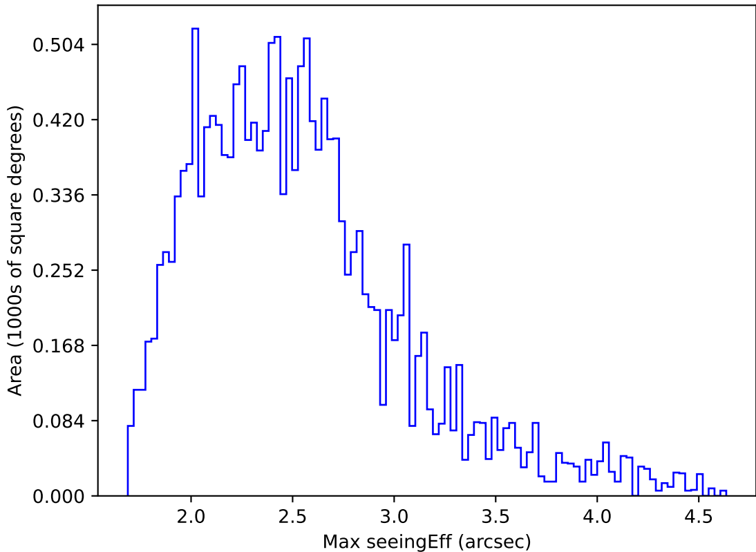
internal_u_expt60_nscale1.1v3.4_10yrs WFD g band: Max seeingEff
