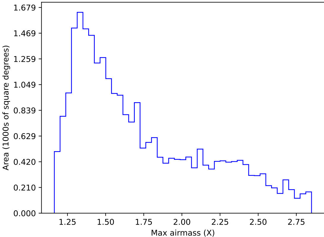
internal_u_expt60_nscale1.1v3.4_10yrs Yr 1 z band: Max airmass
