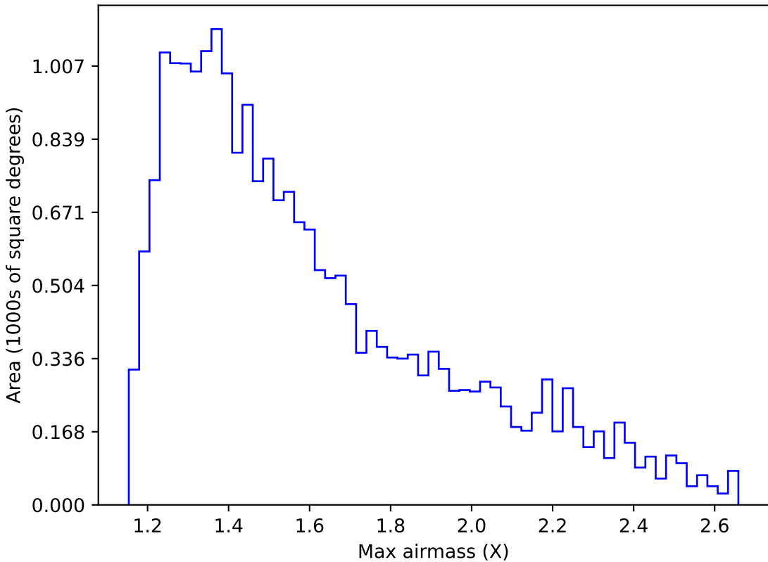
internal_u_expt60_nscale1.1v3.4_10yrs Yr 1 y band: Max airmass
