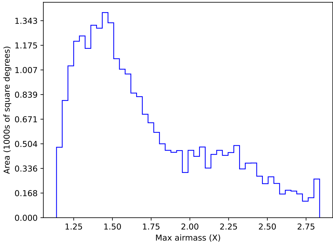
internal_u_expt60_nscale1.1v3.4_10yrs Yr 1 i band: Max airmass
