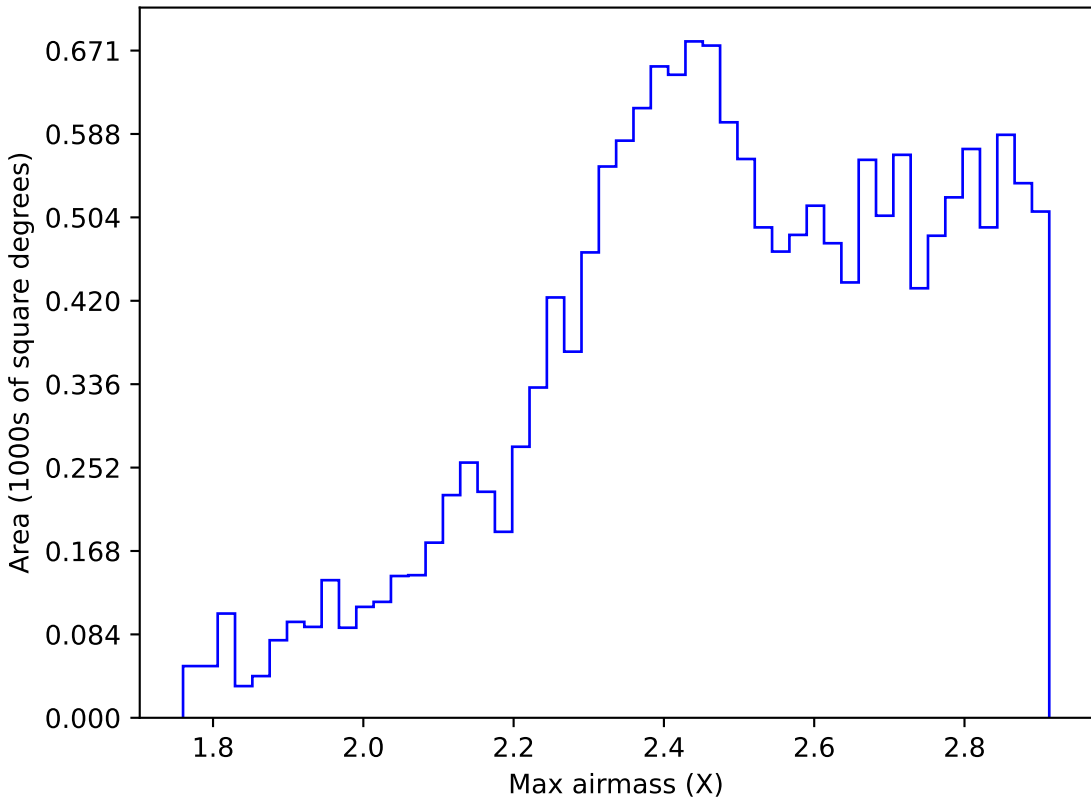
internal_u_expt60_nscale1.1v3.4_10yrs WFD z band: Max airmass
