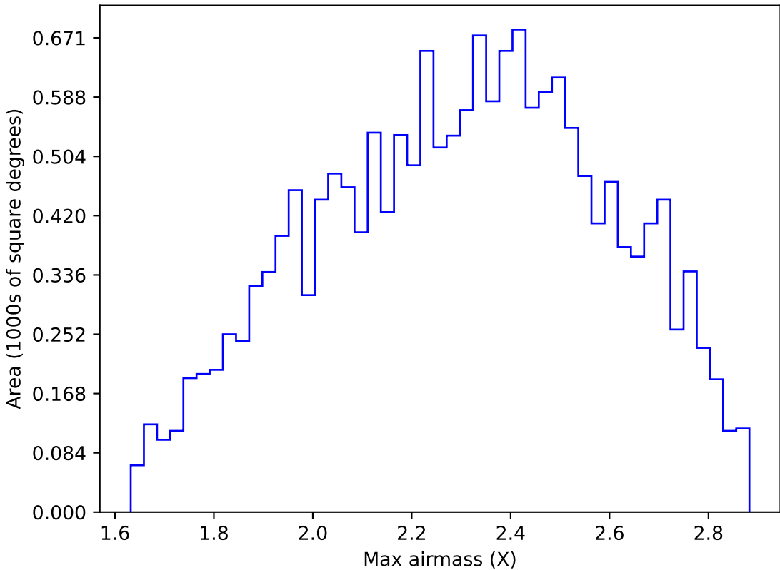
internal_u_expt60_nscale1.1v3.4_10yrs WFD y band: Max airmass
