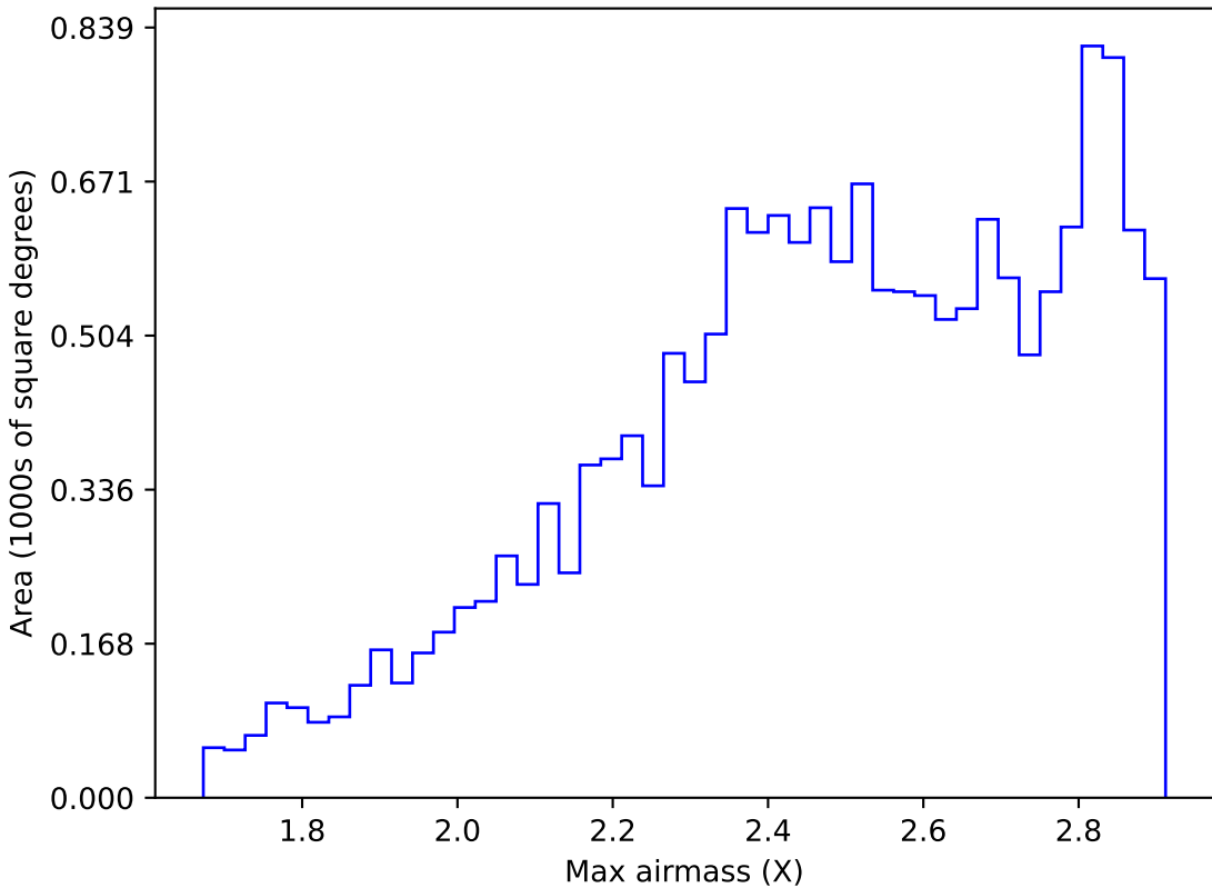
internal_u_expt60_nscale1.1v3.4_10yrs WFD i band: Max airmass
