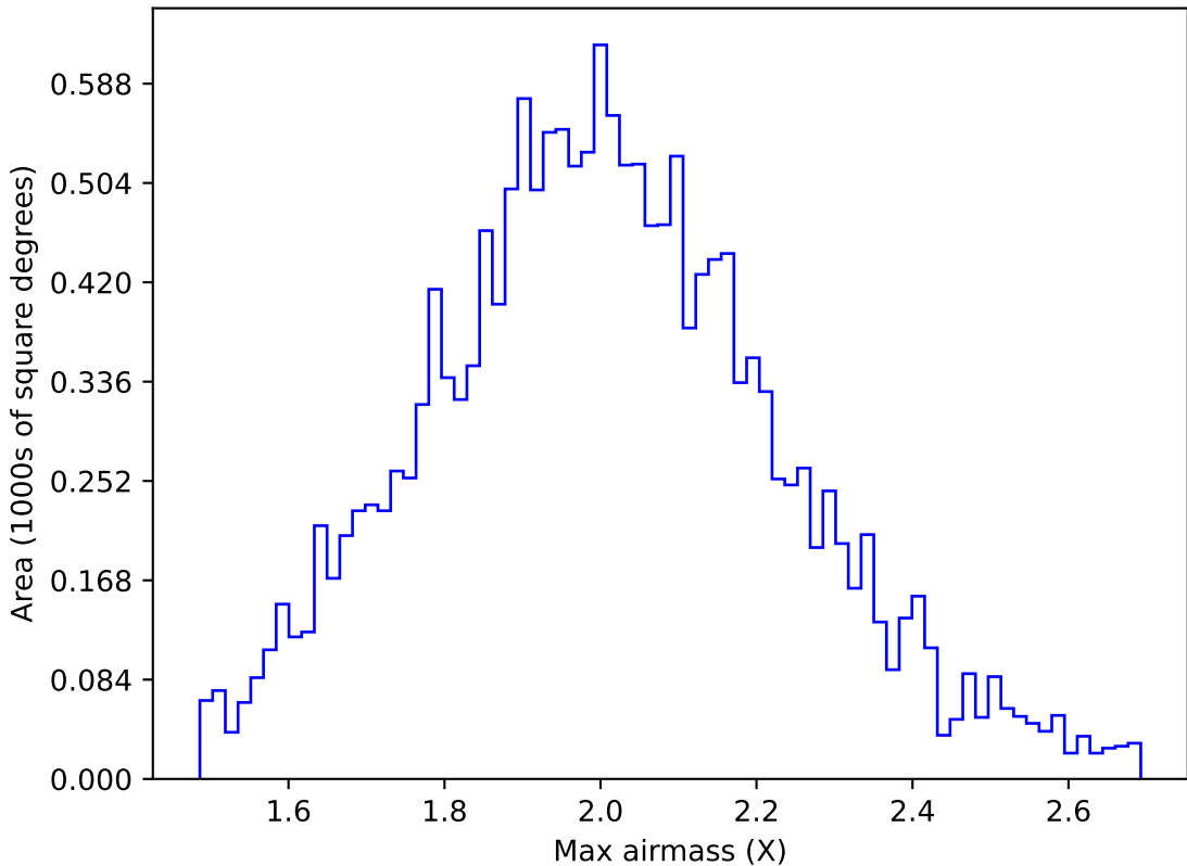
internal_u_expt60_nscale1.1v3.4_10yrs WFD g band: Max airmass
