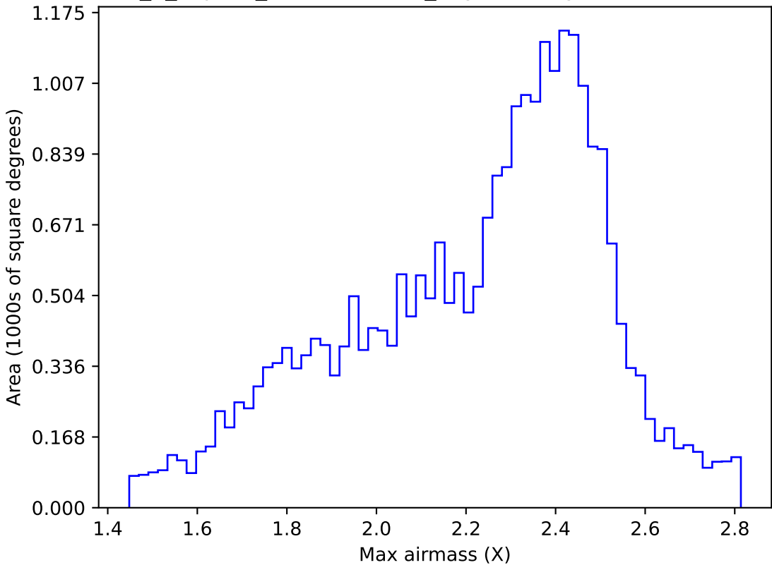
internal_u_expt60_nscale1.1v3.4_10yrs All sky r band: Max airmass
