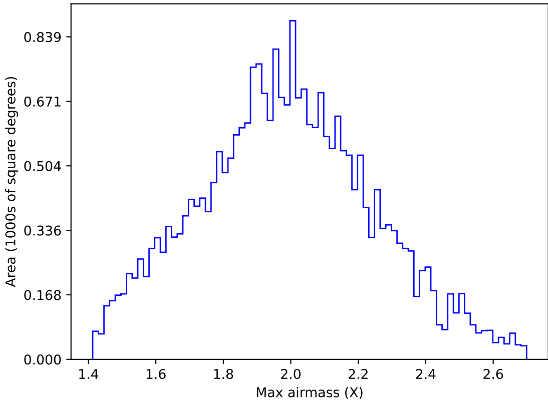
internal_u_expt60_nscale1.1v3.4_10yrs All sky g band: Max airmass
